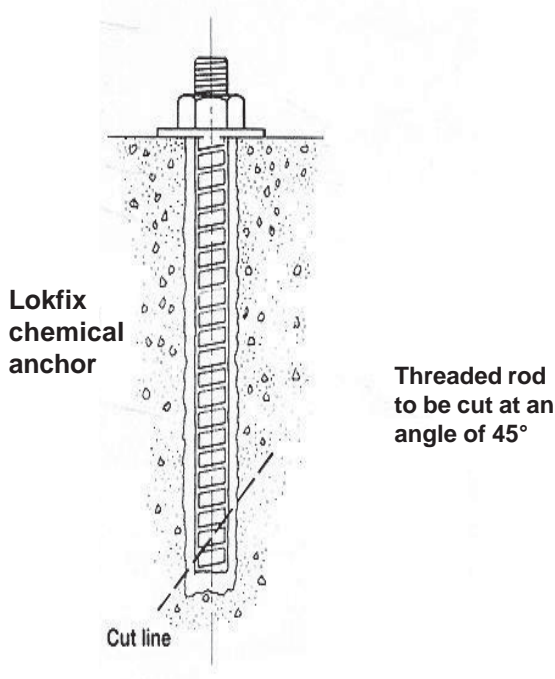
Figure 1: Threaded bar anchored with Lokfix
